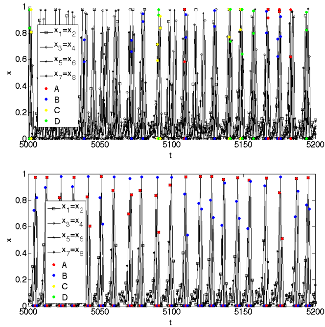
Fig. 8. Temporal dynamics of CNN. Top: Initial condition inside of (11335577). Bottom: Initial condition inside of (11115555). Horizontal axis: Time step t . Vertical axis: CNN output x(t) . The color dots representing the patterns A,B,C,D are superimposed to the value of x(t) when the network retrieved them. k_r = 0.4 , \alpha = 5.0 .
