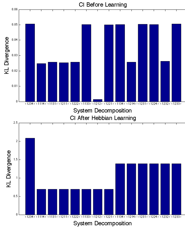
Fig. 16. KL divergence of the system decompositions. Top: Chaotic itinerancy (CI) state before learning. Bottom: Chaotic itinerancy (CI) state after 350 steps of Hebbian learning with learning coefficient \epsilon = 0.01 . Horizontal axis: \langle \dots \rangle represent system decompositions in which correlations between different numbers of elements are set to be independent. e.g. \langle 1212 \rangle corresponds to P^{dec}(y_1, y_2, y_3, y_4) = P(\mathbf{y}^1)P(\mathbf{y}^2) where \mathbf{y}^1 = (y_1, y_3) and \mathbf{y}^2 = (y_2, y_4) . Vertical axis: KL divergence D[P : P^{dec}] . k_r = 0.4 , \alpha = 5.0 , T = 10000 were used for the calculation.
