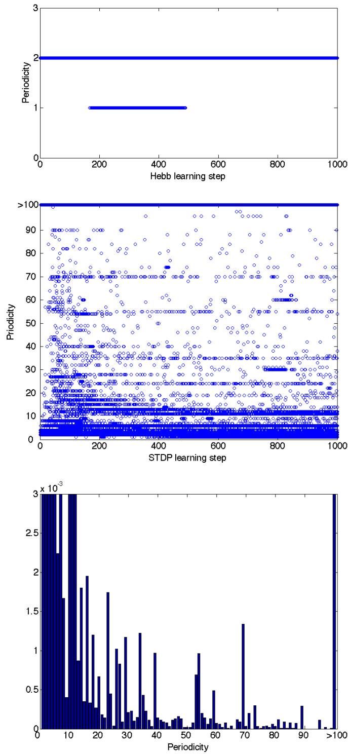
Fig. 13. Periodicity of attractor after autonomous learning. Top: Hebbian learning. Horizontal axis: Time step of Hebb learning. Vertical axis: Periodicity of attractor after the learning. Middle: STDP learning. Horizontal axis: Time step of STDP learning. Vertical axis: Periodicity of attractor after the learning. Bottom: Histogram of periodicity after STDP learning. Horizontal axis: Periodicity of attractor after the learning. Vertical axis: Percentage (Values more than 3.0 \times 10^{-3} are cut off). The periodicity after the learning was judged by resetting k_r = \alpha = 0 and cutting 5000 transient. 100 trials are superimposed for each learning step. Initial conditions were taken randomly.
