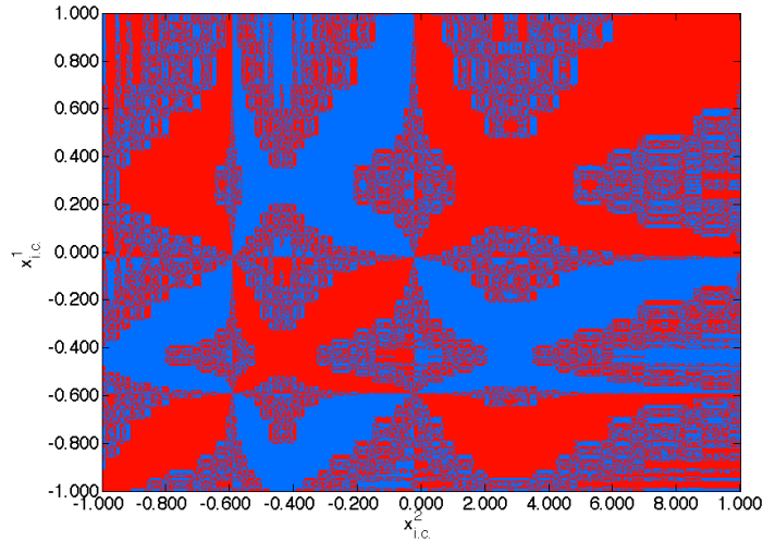
Fig. 11. Basins structure of CNN. Horizontal axis: Value of x_{i,c}^2 . Vertical axis: Value of x_{i,c}^1 . Initial condition were taken inside (11335577) and close to (11331133) as (\eta_1, \dots, \eta_8)^T = (\zeta_1, \dots, \zeta_8)^T = (x_{i,c}^1 + \delta, x_{i,c}^1 + \delta, x_{i,c}^2 + \delta, x_{i,c}^2 + \delta, x_{i,c}^1 - \delta, x_{i,c}^1 - \delta, x_{i,c}^2 - \delta, x_{i,c}^2 - \delta)^T with \delta = 1.0e - 6 . The red region is where the orbits reach to the neighbor of the patterns A \Rightarrow B first, while the blue region reach to the neighbor of the patterns C \Rightarrow D first. x_{i,c}^1 and x_{i,c}^2 were taken for each 0.002 step with parameters k_r = 0.4 and \alpha = 5.0 .
