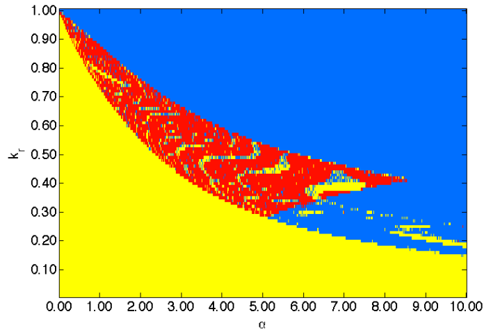
Fig. 5. Wandering range among memorized patterns of CNN. Horizontal axis: \alpha . Vertical axis: k_r . The blue region is where the dynamics visit none of the patterns A, B, C, D. The yellow region is where the dynamics visit only either pair of patterns A=B or C=D. The red region is where the dynamics visit both pairs of patterns A=B and C=D. After cutting 5000 transient, 10000 steps were used to calculate the wandering range at each 0.01 step of k_r and \alpha . Initial conditions were taken randomly.
