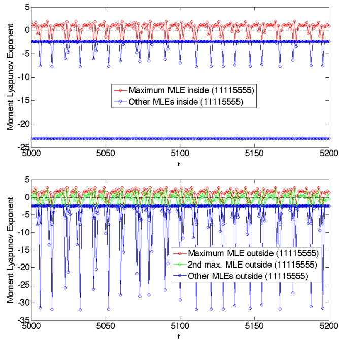
Fig. 10. Temporal dynamics of moment Lyapunov exponents with initial condition inside of (11115555). Top: Moment Lyapunov exponents to the direction inside of (11115555). Bottom: Moment Lyapunov exponents to the direction outside of (11115555). Horizontal axis: Time step t . Vertical axis: Moment Lyapunov exponent. k_r = 0.4 , \alpha = 5.0 .
