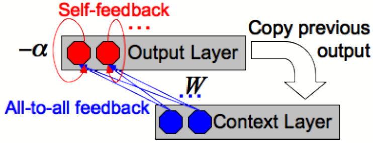
Fig. 1. Architecture of CNN.
