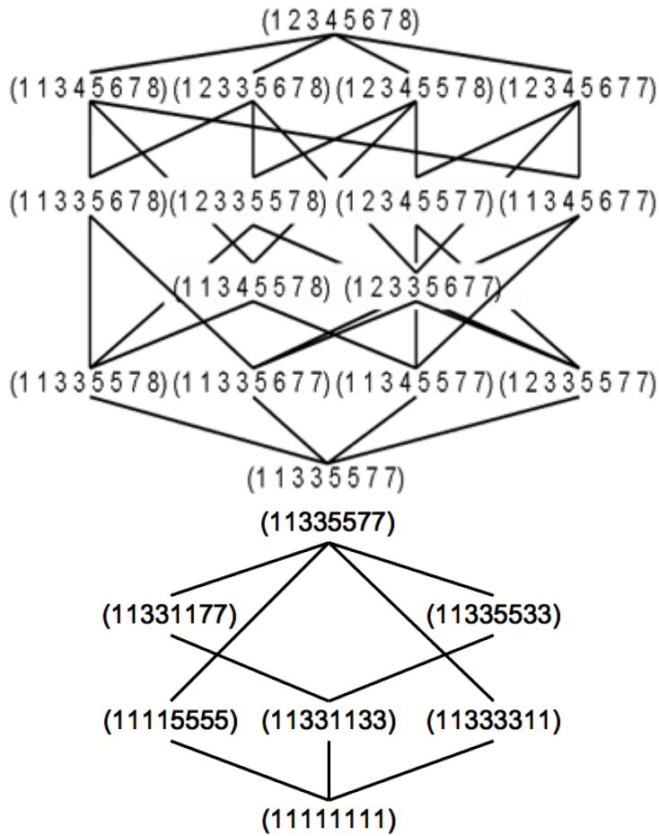
Fig. 2. Invariant subspaces of CNN in the defined setting. Top: Above (11335577). Bottom: Below (11335577). The lines denote inclusion relation. Although there exist actually 76 invariant subspaces, for simplicity only those in the above/below hierarchy of (11335577) are shown.
