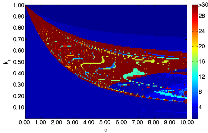
Fig. 3. Periodicity of CNN. Horizontal axis: \alpha . Vertical axis: k_r . After cutting 5000 transient, periodicity was judged with the tolerance of 1.0e-6 for each neuron output. More than 30 periodic orbit is depicted in brown. After cutting 5000 transient, 10000 steps were used to calculate the periodicity at each 0.01 step of k_r and \alpha . Initial conditions were taken randomly.
