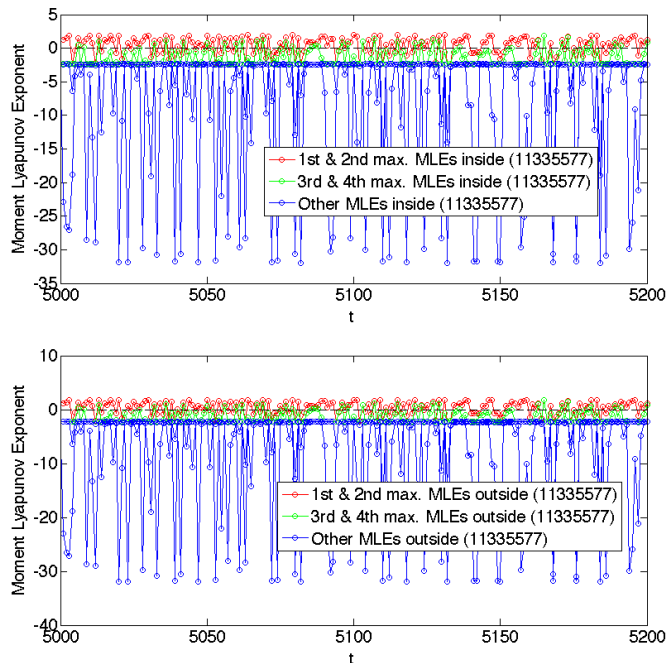
Fig. 9. Temporal dynamics of moment Lyapunov exponents with initial condition inside of (11335577). Top: Moment Lyapunov exponents to the direction inside of (11335577). Bottom: Moment Lyapunov exponents to the direction outside of (11335577). Horizontal axis: Time step t . Vertical axis: Moment Lyapunov exponent. k_r = 0.4 , \alpha = 5.0 .
