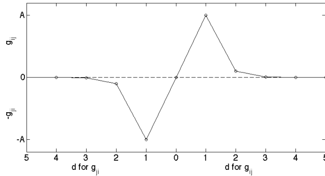
Fig. 12. STDP rule for discrete time CNN. Horizontal axis: Spike time interval d . Vertical axis: Modification to w_{ij} defined in equation (62). k_{STDP} = 0.1 .
