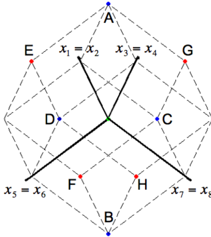
Fig. 14. Possible emergent attractors after Hebb learning. The arrows are four-dimensional coordinates (x_1 = x_2, x_3 = x_4, x_5 = x_6, x_7 = x_8)^T of the CNN output inside of (11335577) . The blue points are memorized patterns A, B, C, D. The red points E, F, G, H are possible emergent two-periodic attractors, and are situated at the equidistance points from A \rightleftharpoons B and C \rightleftharpoons D . Only two-periodic patterns E \rightleftharpoons F and G \rightleftharpoons H are possible to emerge. The green point is the divergent case that corresponds to the fix point (1, 1, 1, 1)^T .
